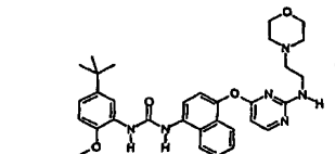
1-(5-tert-Butyl-2-methoxy-phenyl)-3-{4-[2-(2-morpholin-4-yl-ethylamino)-pyrimidin-4-yloxy]-naphthalen-1-yl}-urea;
